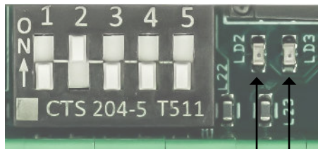
DIP-bryter
